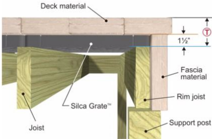
End of Joist (Front) View
